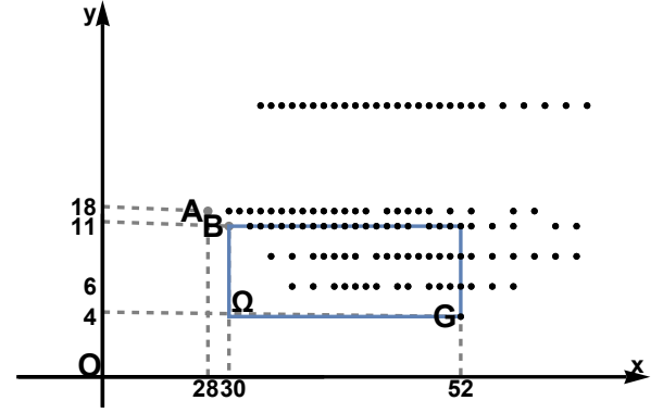
Fig. 2. Partial MCPF and the rectangle area \Omega for the example network N_1 . The POST that represent the class P_1 is denoted with A, and the POST that represent the class P_2 is denoted with B. The barrier tree is denoted with G
