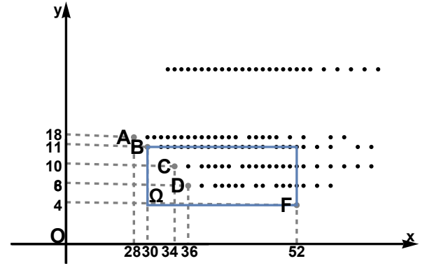
Fig. 3. MCPF for the example network N_1 . The POSTs that represent the classes P_1 to P_5 are denoted with A, B, C, D and F respectively
