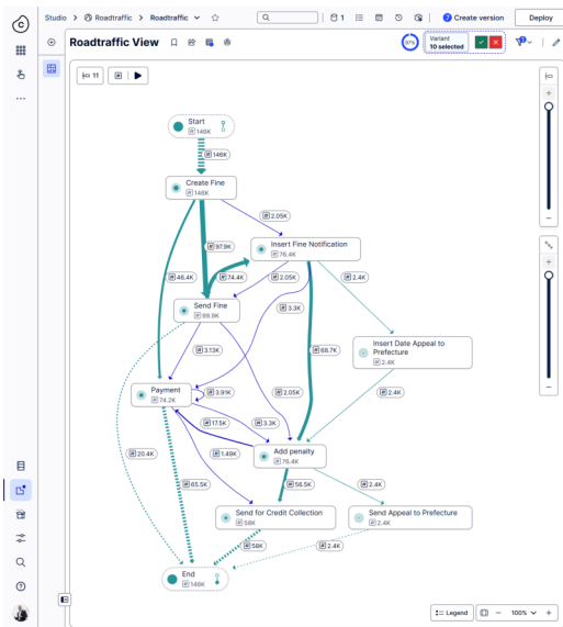
Fig. 2. Process model based on the top 10 variants covering 97% of the road traffic fines.
