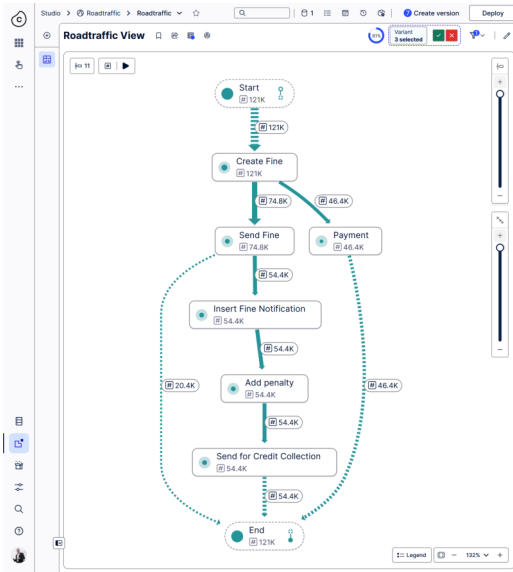
Fig. 1. Process model based on the top 3 variants covering 81% of the road traffic fines.
