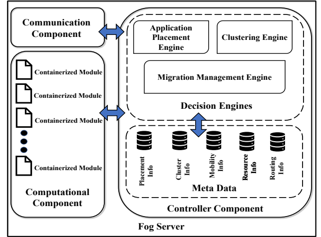
Figure 4: A view of fog server architecture
