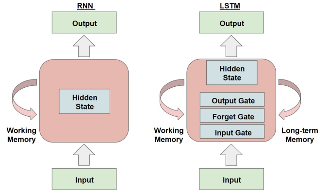
Fig. 6. Architecture of RNN (left) vs LSTM (right).
